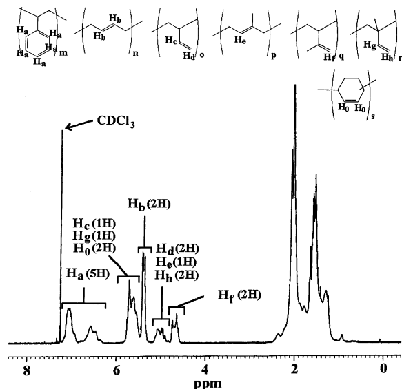
Figure 10. ^1\text{H} NMR of the fractionated PS- b -PB- b -PI- b -(1,4-PCHD) (19/20/22/39, Table 4) quaterpolymer in \text{CDCl}_3 at 30 ^\circ\text{C} .
