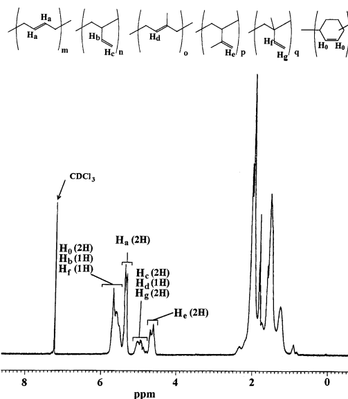
Figure 8. ^1\text{H} NMR of the fractionated PB- b -PI- b -(1,4-PCHD) (25/29/46, Table 3) terpolymer in \text{CDCl}_3 at 30\text{ }^\circ\text{C} .
