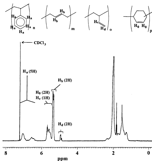
Figure 4. ^1\text{H} NMR of the PS- b -PB- b -(1,4-PCHD) (17/43/40, Table 3) terpolymer in \text{CDCl}_3 at 30 ^\circ\text{C} .
